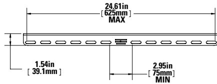
WALL PLATE
