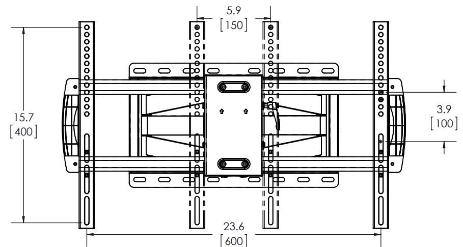
TV INTERFACE
