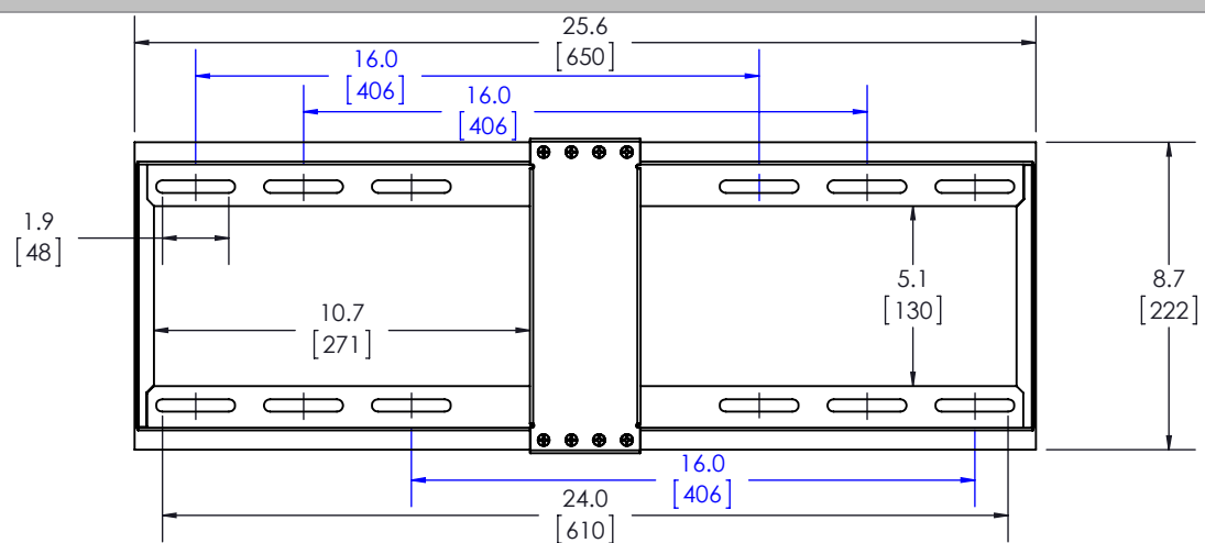
WALL PLATE
